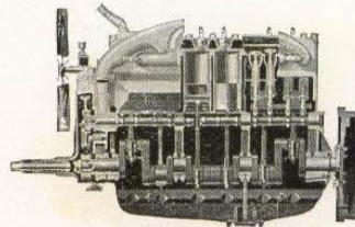
Long ten-inch completely machined connecting rods; large, rigid, completely machined crankshaft with large bearings; oil reservoir.
