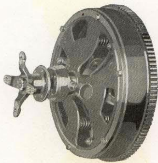
The single plate dry disc clutch makes gear shifting quiet and easy. Clutch brake serves to prevent spinning of transmission gears after clutch is disengaged.
